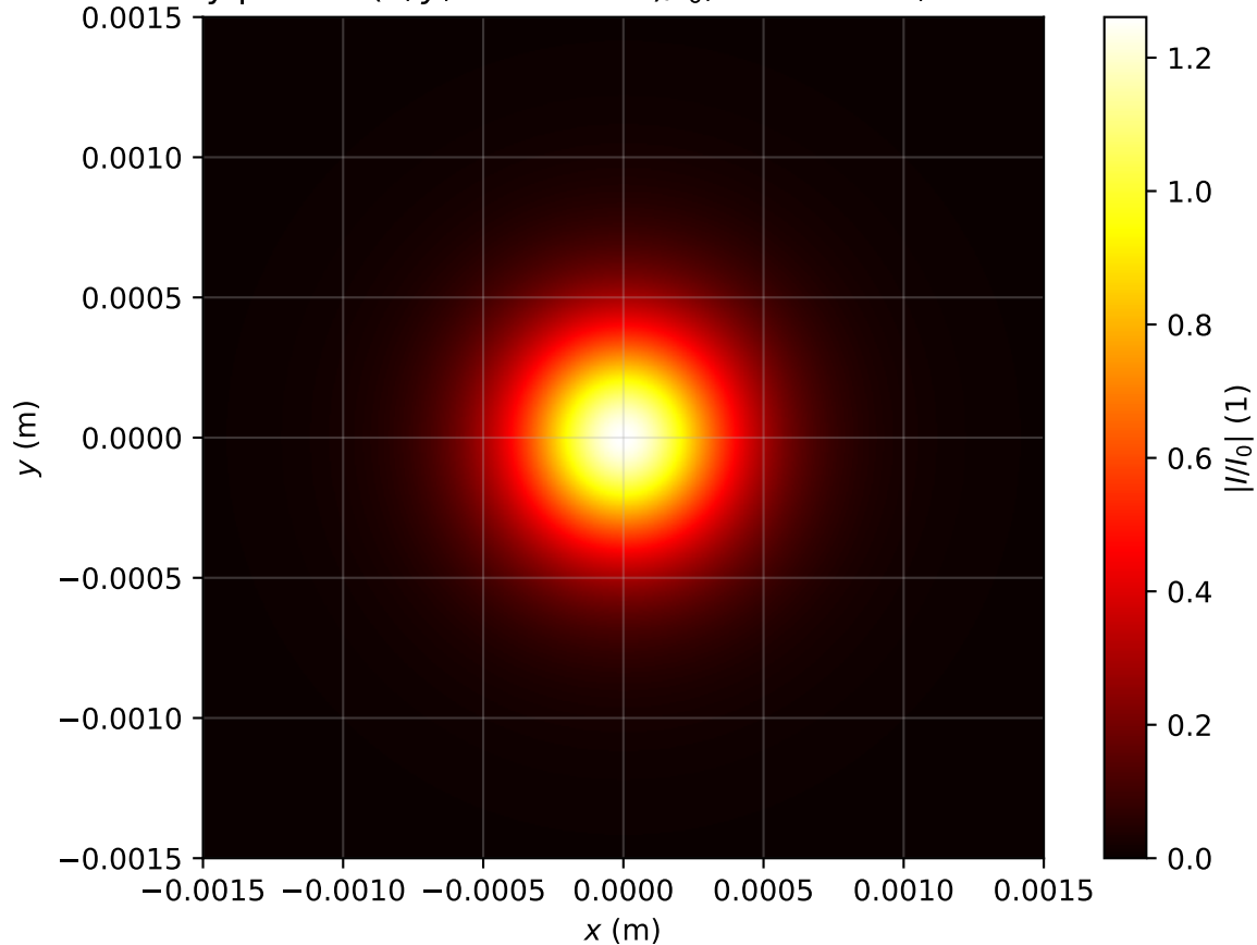
Intensity profile I(x, y, z = 2.309m)/I_0 , Pin=0.8Pcr, artificial time
